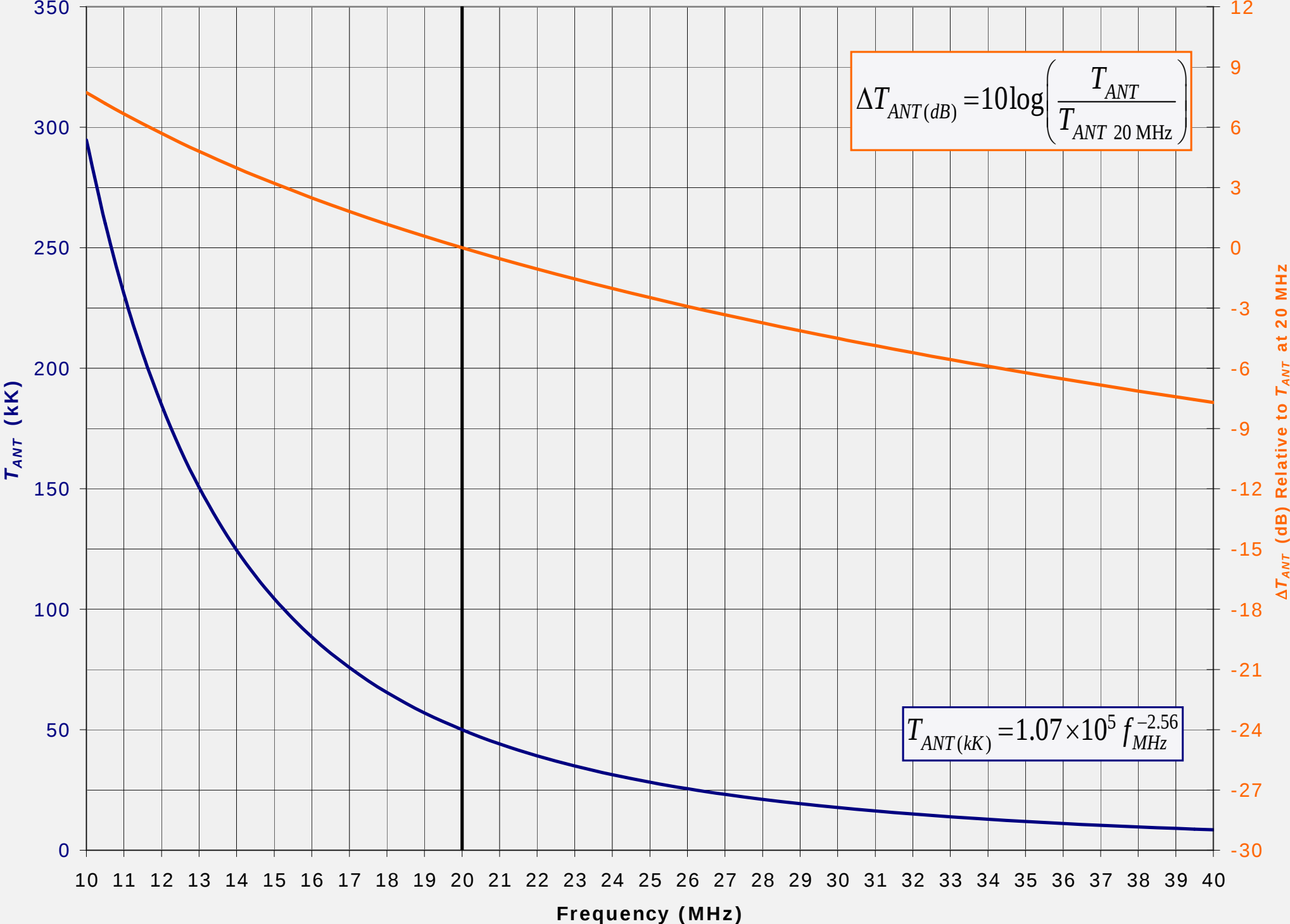
Polar Galactic Background, Wide Beam, T_{ANT} Model and \Delta T_{ANT}
