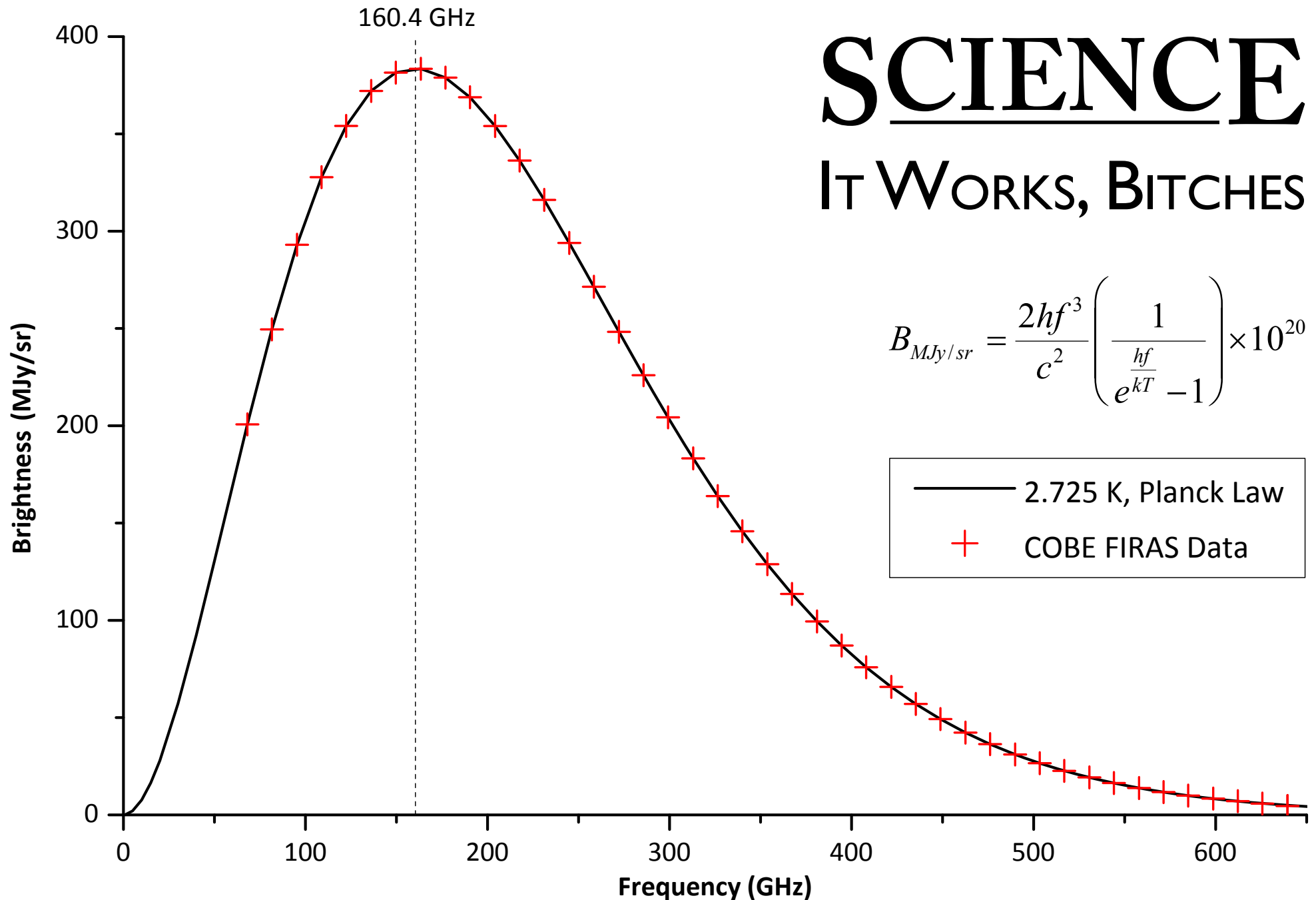
CMBR Spectrum (COBE FIRAS Data) and 2.725 K Blackbody Spectrum
