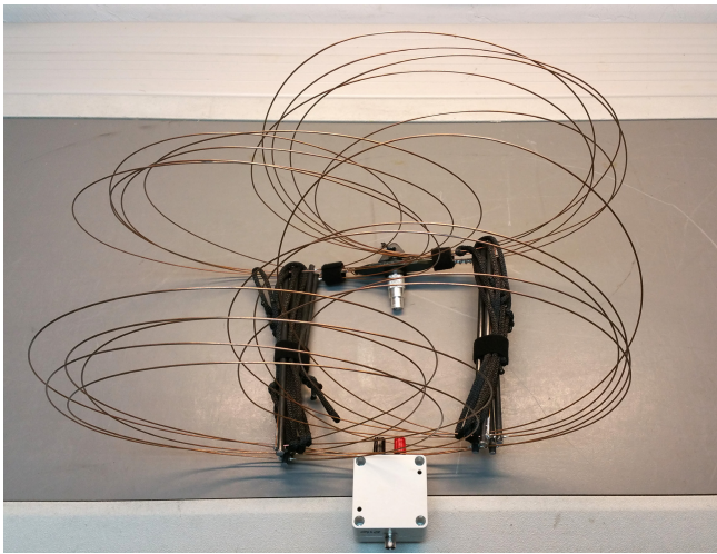
Figure 3 – The 30' TFD element coiled for storage. 1
