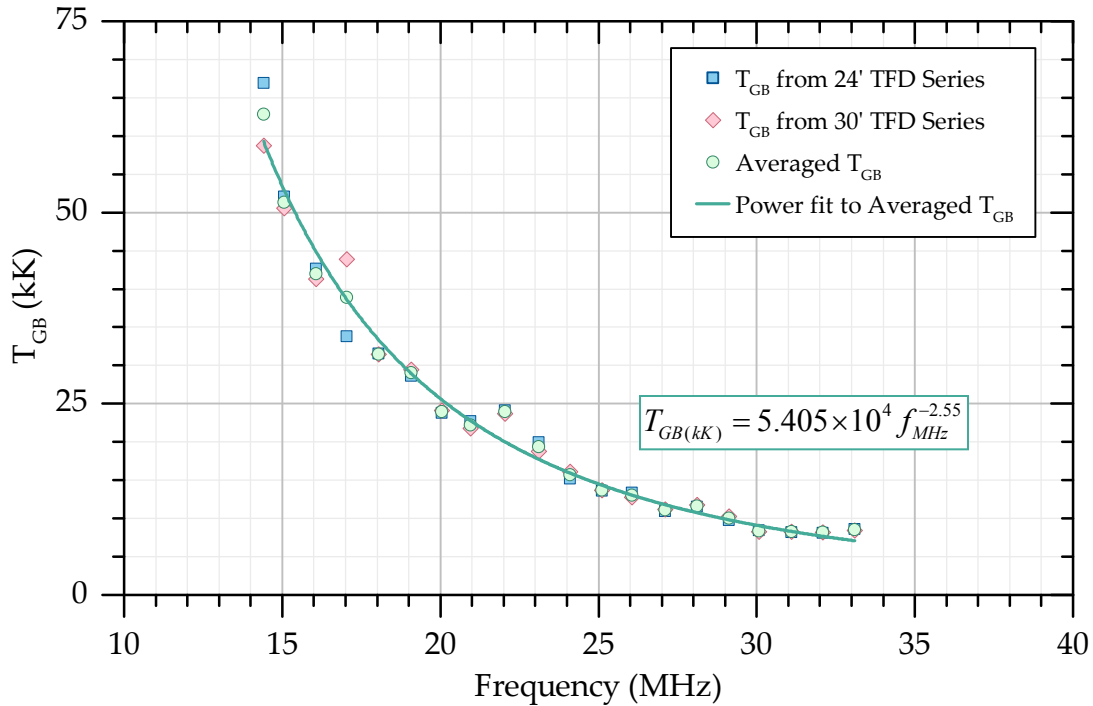
Plot 2 – Galactic background antenna temperatures measured using the reference dipoles. One series represents measurements used for comparison with the 24' TFD, the other represents measurements used for comparison with the 30' TFD. The series were averaged at each frequency and a power function fitted to the averages using Origin 9 software. The result shows a spectral index of -2.55. The known spectral index of the polar galactic background is -2.56. 5 Agreement with the accepted value shows that the impact of any radio frequency interference (RFI) on the efficiency analysis as a whole is not significant, RFI being expected to have a spectrum different than that of the GB. RFI may have had a greater impact at individual test frequency measurements, but none appear to have been greatly affected by RFI. The known 20 MHz temperature of the galactic background is 50 kK. 5 The measured temperatures are thus 3 dB colder than expected. It is possible this difference is due to the dipole antennas being situated over poor natural ground without a wire ground screen; however, there may be other contributing factors presently unknown.
