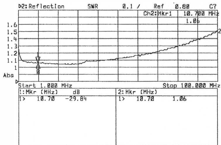
10/7 MHz IF AMP #1 OUTPUT SWR
