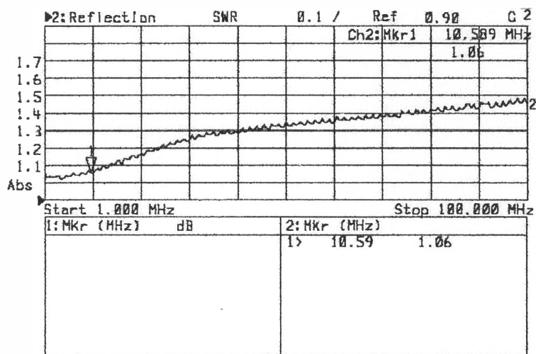
10.7 MHz Diplexer, 2N-5109 Amp, 6 dB Pad Output VSWR
