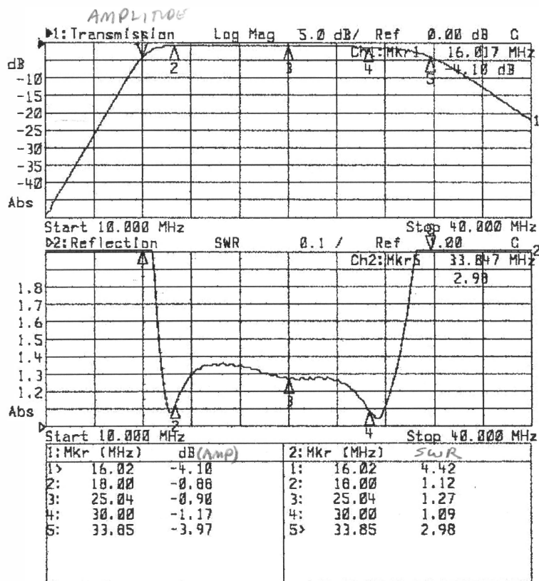
18 - 30 MHz bandpass filter amplitude response and VSWR
